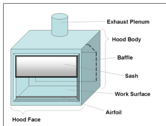
Figure IV-III. Fume Hood
